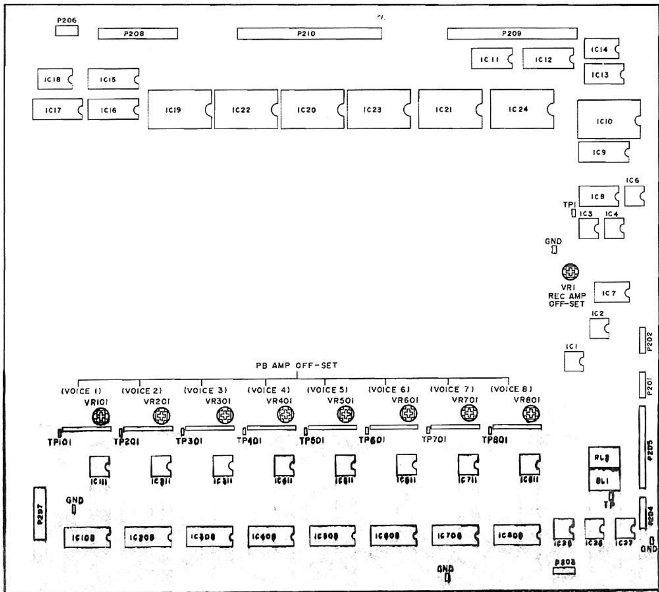
Fig. 5-1 Adjustment points of VOICE PCB
