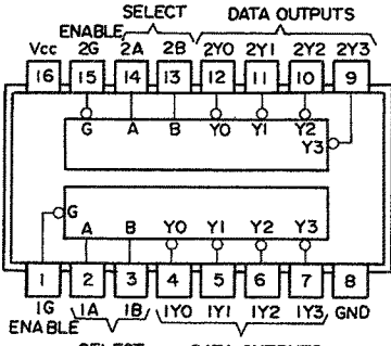
'LS139, (EACH DECODER/DEMULPLEXER) FUNCTION TABLE
