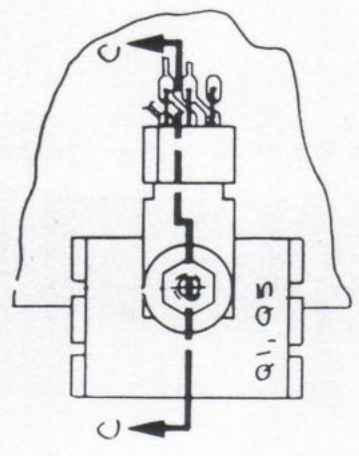
MOUNTING ALTERNATE TRANSISTOR D40D4
