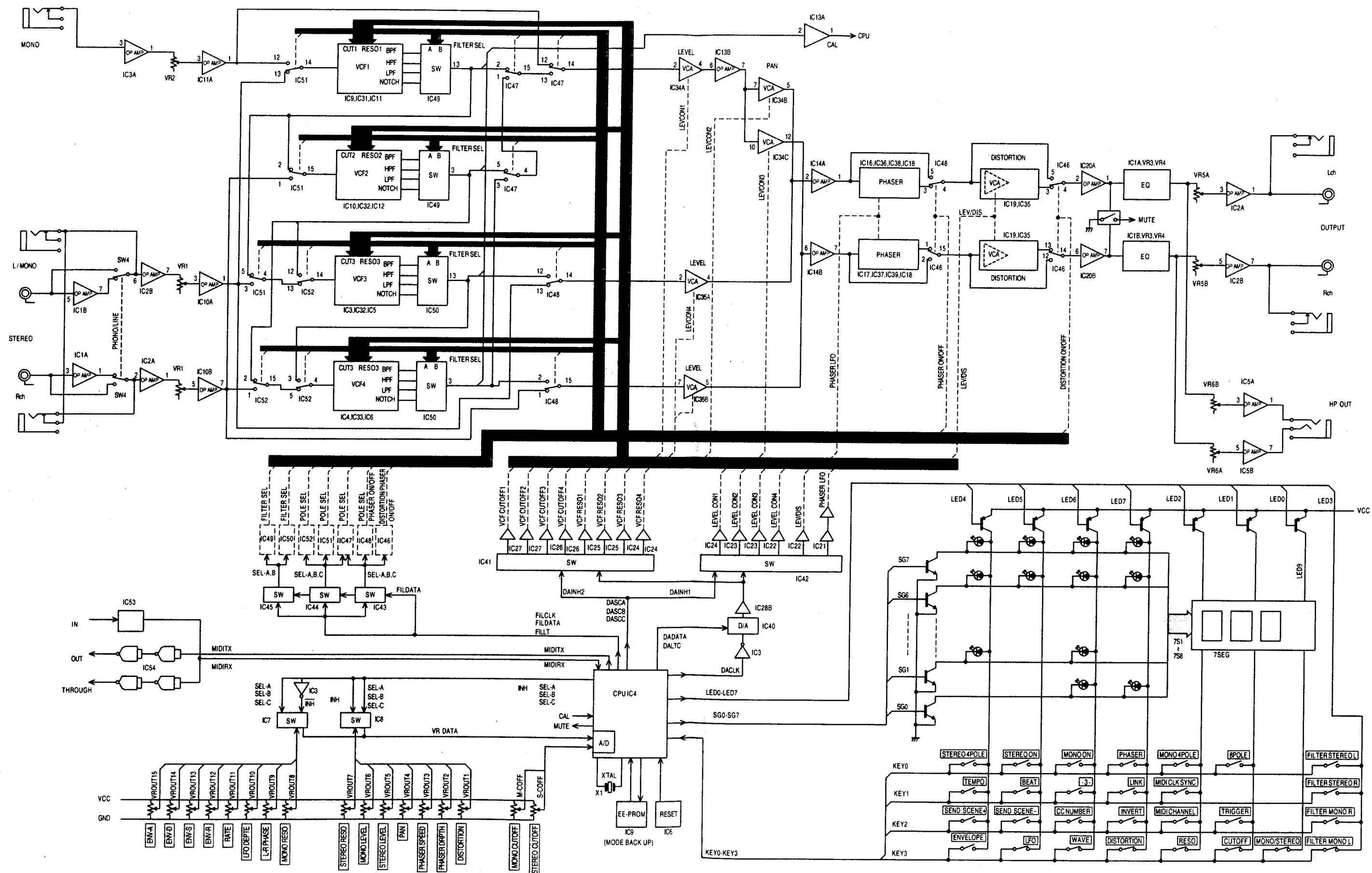
MF42 BLOCK DIAGRAM
